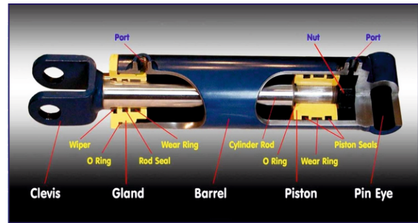
Hydraulic Cylinder Showing internal components
